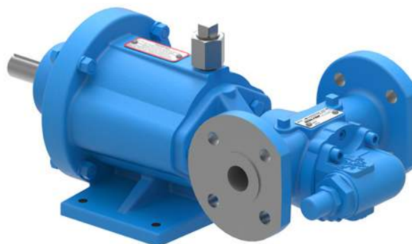
GG893 MD-B40B, bearing carrier, footed bracket, and mounted pump with flanged ports (shown with optional temperature probe connection)
