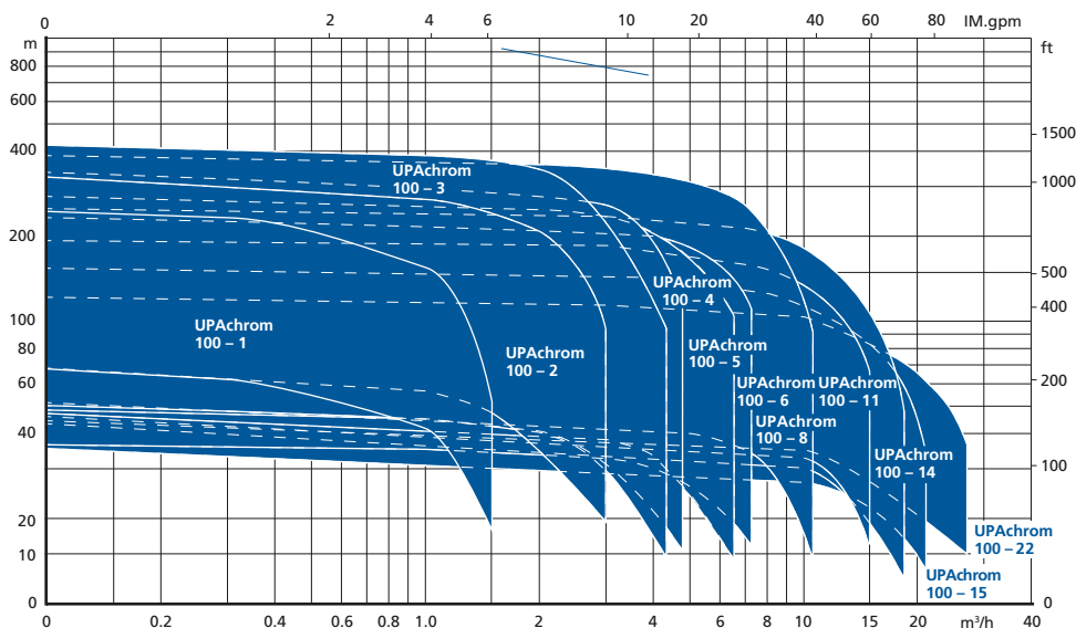
Characteristic curves UPAchrom 100CN (60 Hz)
